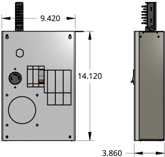
T225-C-10-OB-L520R-G
